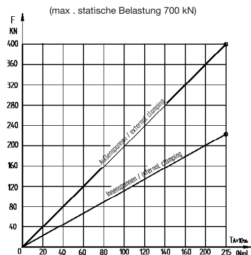
Mechan. Spannspindel "MSPD 120"
